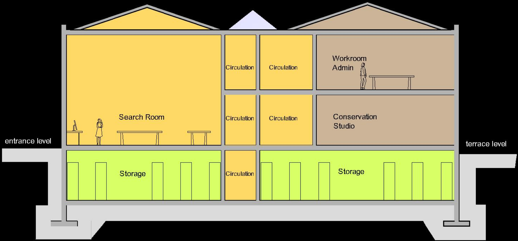
Outline Section
