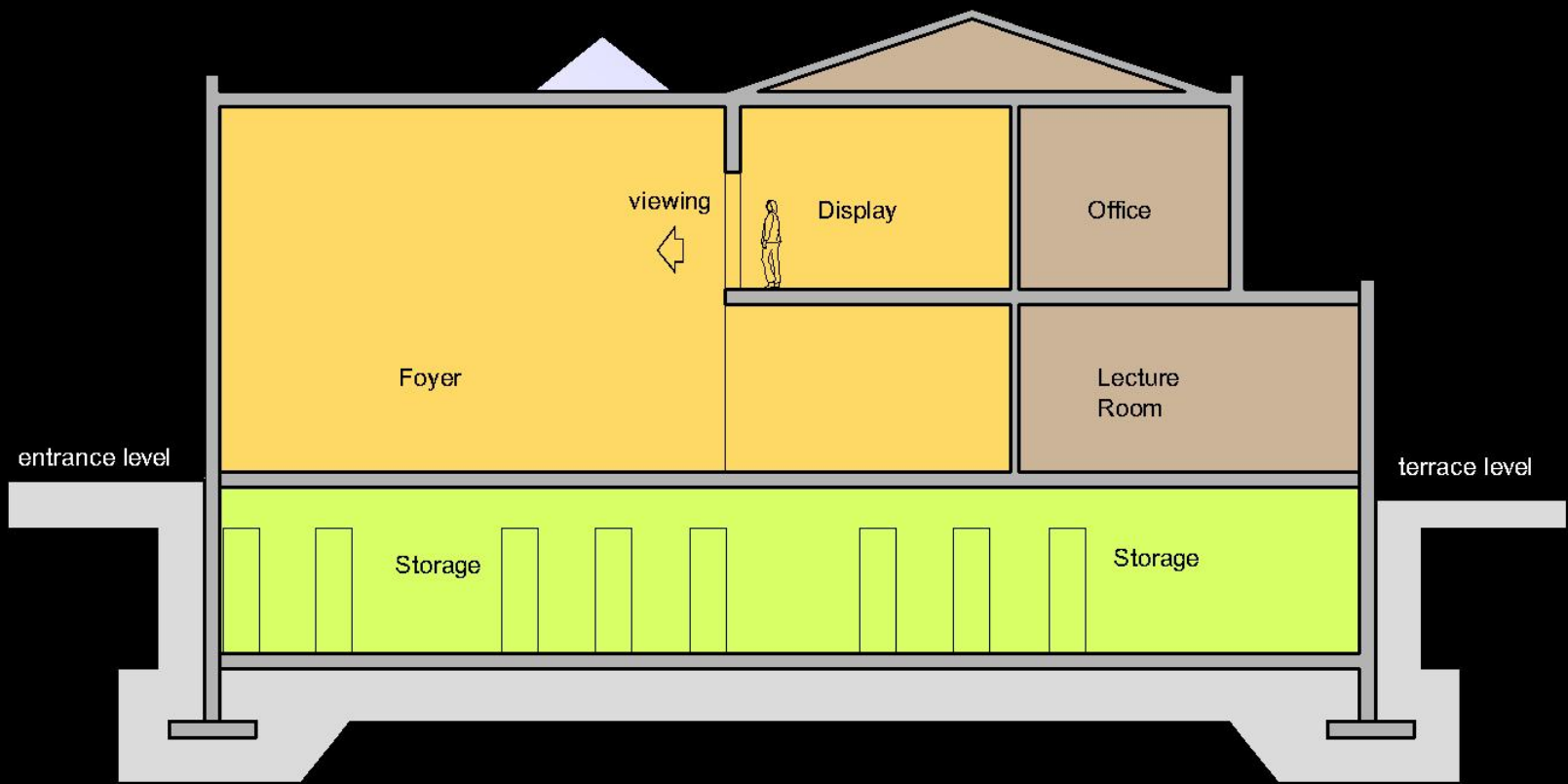
Outline Section
